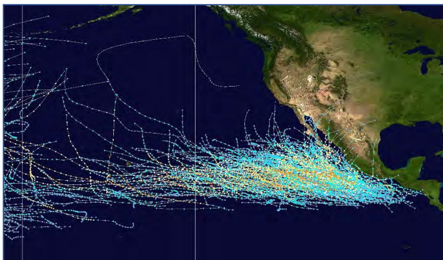
Figure 23: Eastern Pacific tropical cyclone tracks from 1980-2005.
