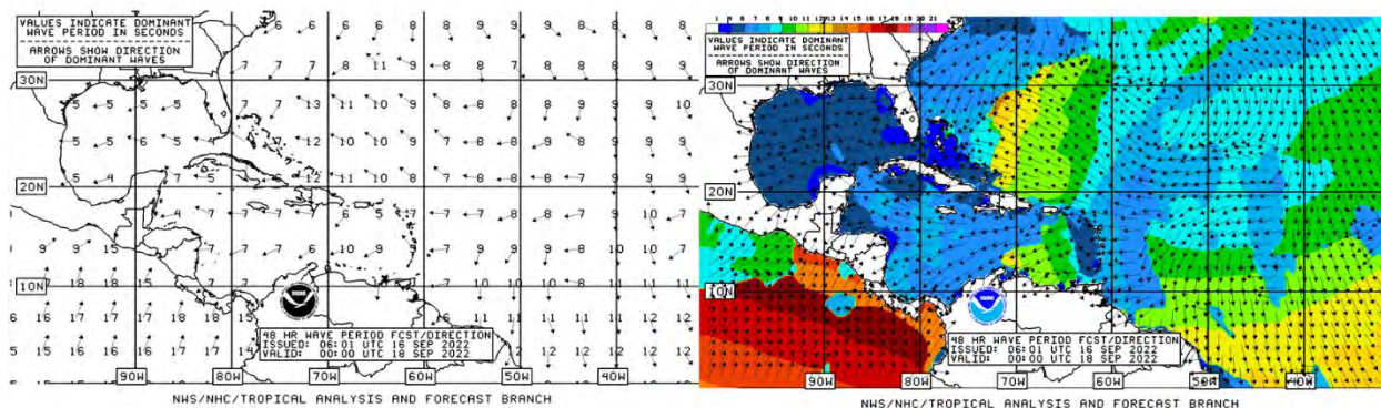
Figure 55: 48-hour Wave Period/Direction Forecast in both black-and-white and color.
