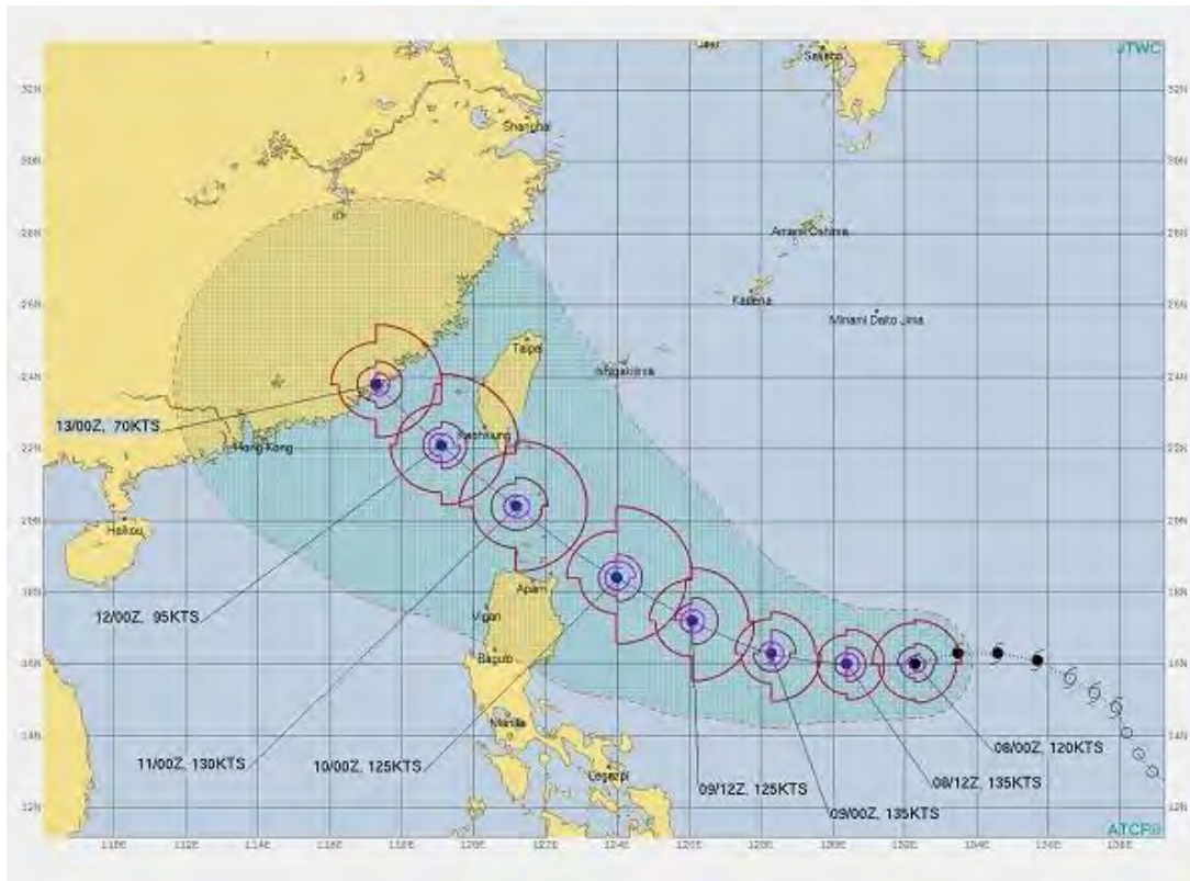
Figure 59: JTWC Warning Graphic.
