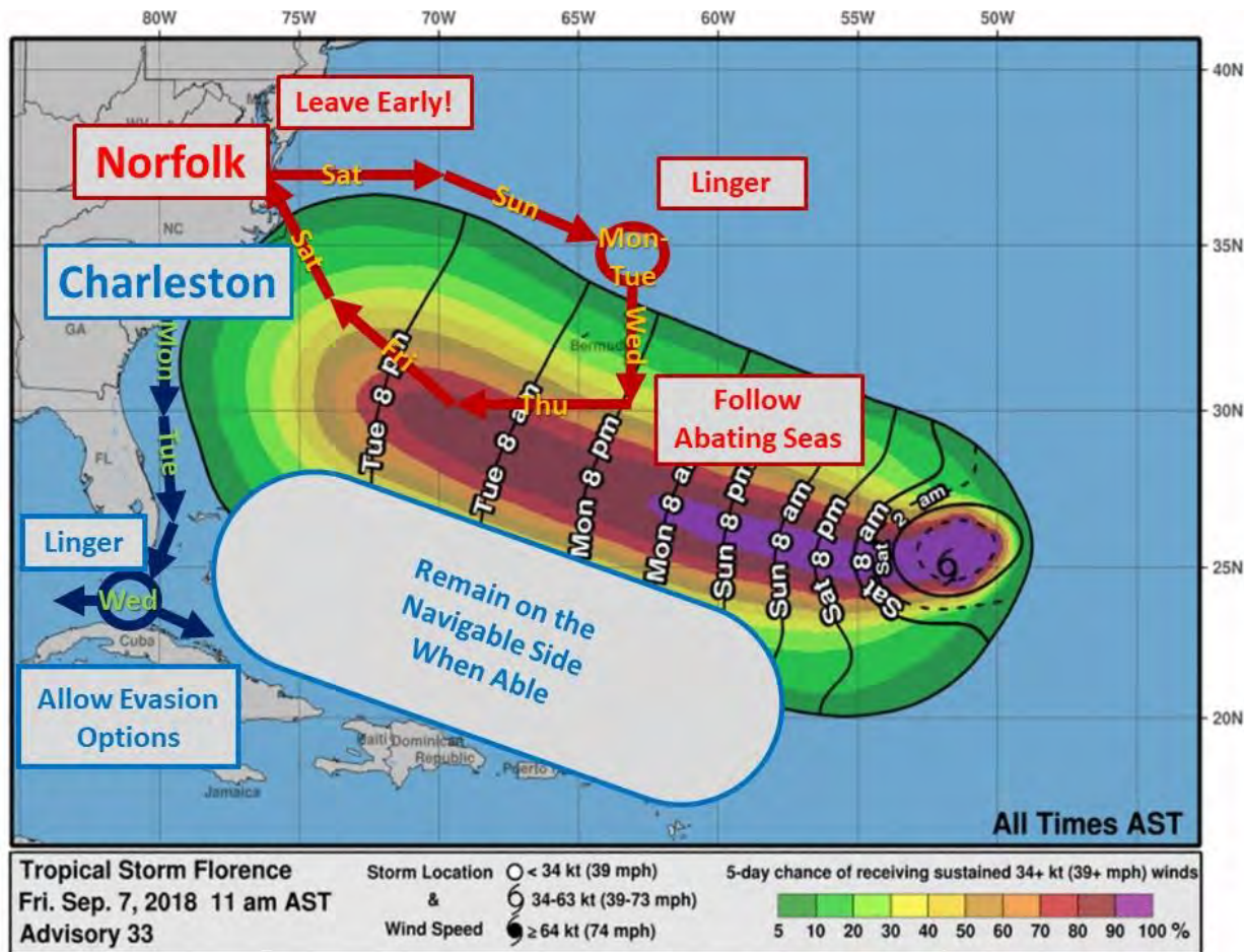
Figure 65: Example Sortie tracks from Norfolk, VA (red) and Charleston, SC (blue) based on the Probability/Arrival Time of Tropical Storm Force Wind graphic with guidelines to follow. At this time, Florence was expected to make landfall early Friday somewhere in the Carolinas as a major hurricane.
