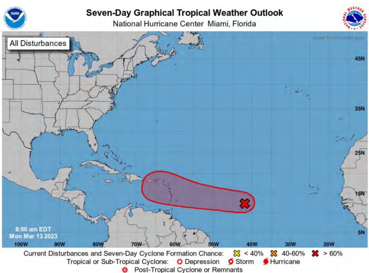
Figure 47: An example 7-day 12 Graphical Tropical Weather Outlook.
