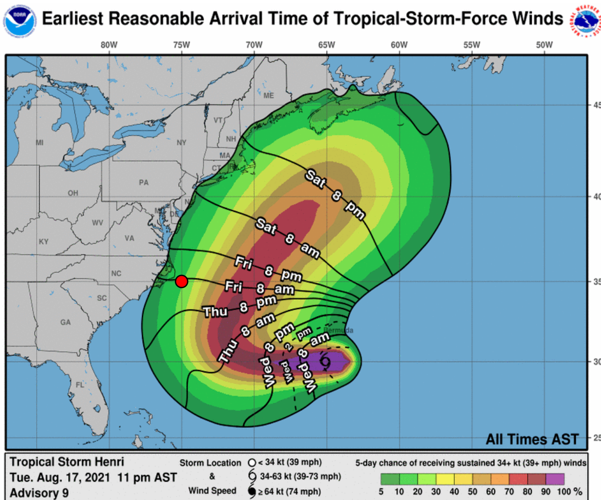
Figure 46: Earliest Reasonable Arrival Time of Tropical Storm Force Winds graphic (black lines) with the probabilities underlaid (colors). For example, a ship off Cape Hatteras at 35N75W has a 20% chance of receiving tropical storm force winds. If these winds occur, the earliest reasonable time they will begin is around 8 am AST Friday. Specifically, there is only a 10% chance they will begin before this time.
