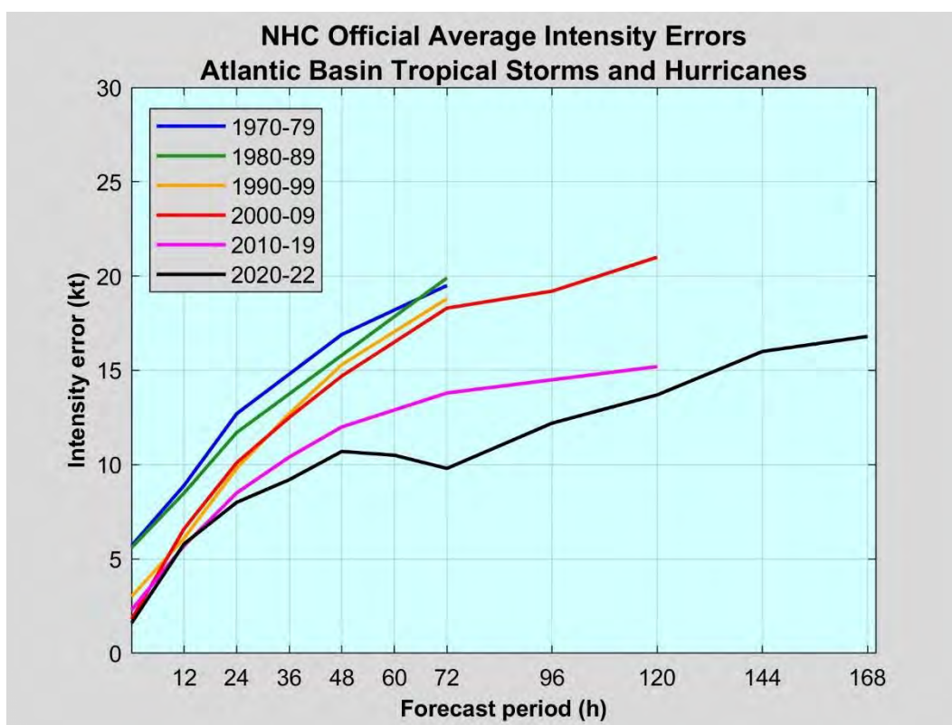
Figure 36: NHC intensity errors by decade from 1970-2022 for the North Atlantic. After several decades with little improvement, errors have decreased in recent years.
