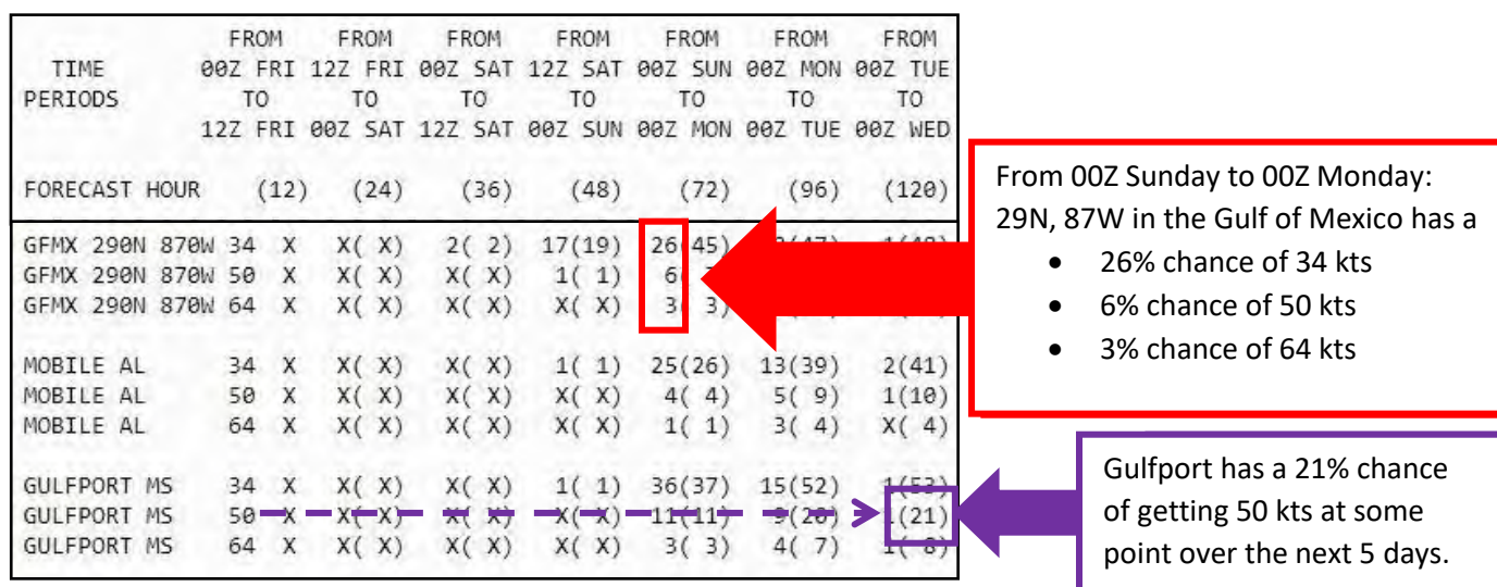
Figure 39: Annotated Tropical Cyclone Surface Wind Probabilities (PWS).
