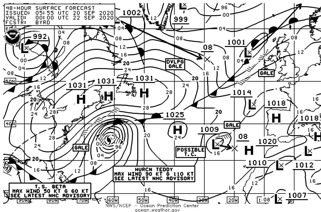
Figure 54: 48-hour Surface Forecast.
