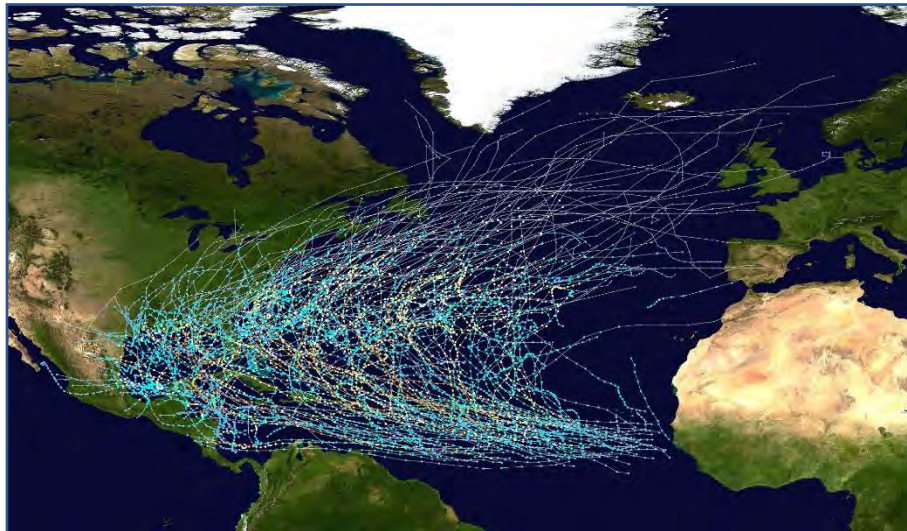
Figure 21: North Atlantic tropical cyclone tracks from 1980-2005.
